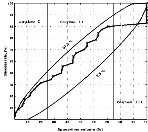
Figure 2: Receiver Operating Characteristic Curve calculated for “M8” for the 35 events with M \geq 7.5 (1985-1996) shown in Figure 1. The two smooth curves labeled 2.5% and 97.5% define a 95% confidence interval based on the null hypothesis that the algorithm samples the space-time according to a uniform probability density. An ROC curve excursion above this region is diagnostic of an algorithm that performs better than random. Similarly, an ROC curve that wanders below this region indicates an algorithm performance worse than random. This diagram shows the population of events used here to be tri-modal in terms of M8 performance. For regime I (11 events) M8 performs somewhat better than random; for regime II (17 events) M8 performs no better than random, and for regime III (7 events) no successful prediction could be made.
